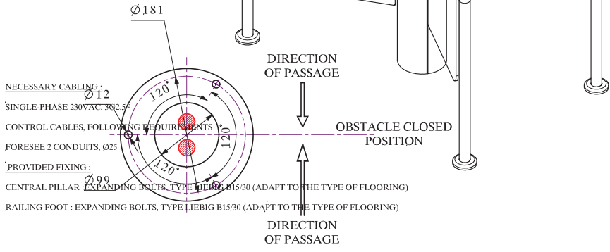
FLOOR FIXING DETAIL
