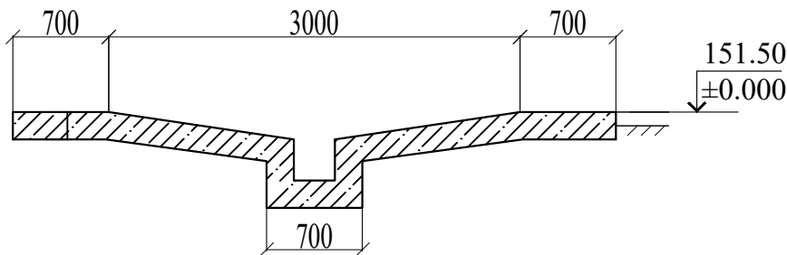
Section 2-2
