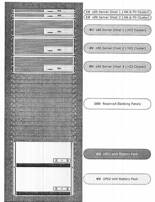
19" 42U Rack #2 Rack placement front view
