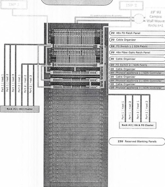
19" 42U Rack #1 Wiring & rack placement front view
