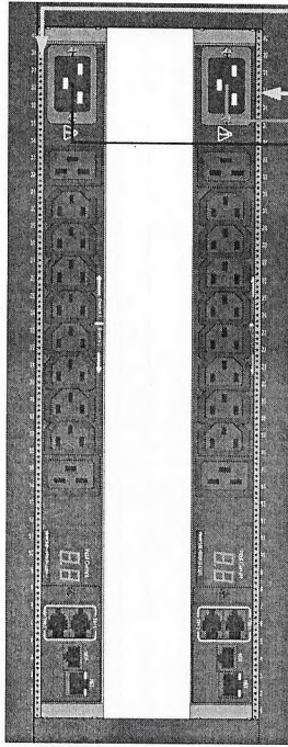
19" 42U Rack #1 Rack power distribution rear view
