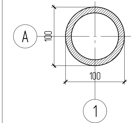
Section 1-1 Sc. 1:10
