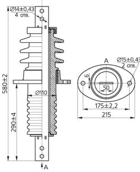
ИПУ-10/630
