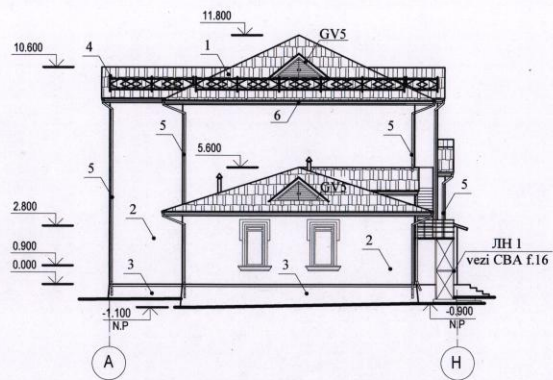
Fatada A - H
