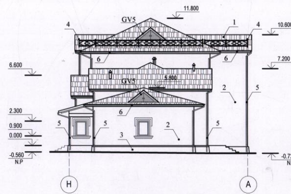
Fatada H - A
