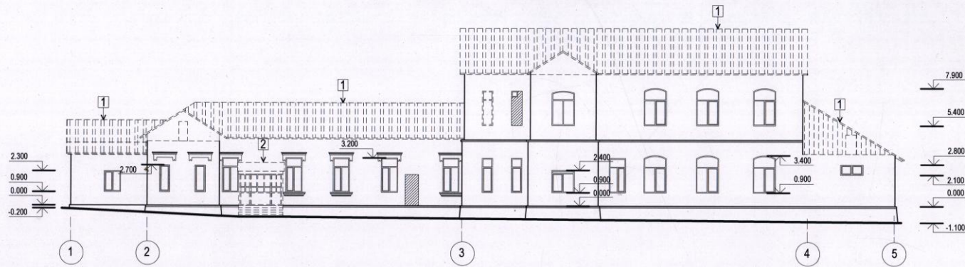
Fatada 1 - 5 demontare ( Relevu )
