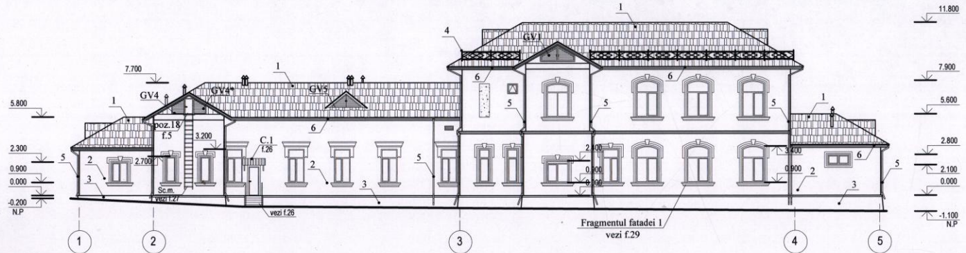
Fatada 5 - 1
