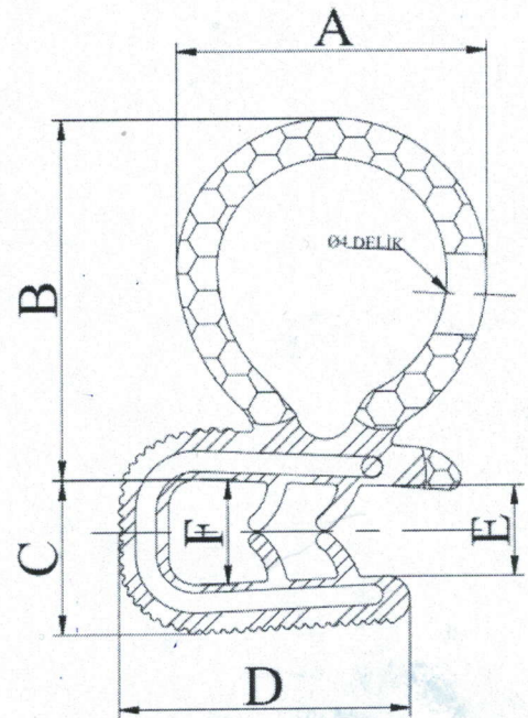
Technical Drawing
