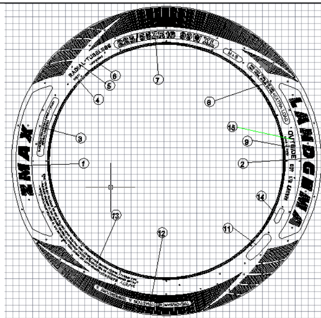
Lower mold
