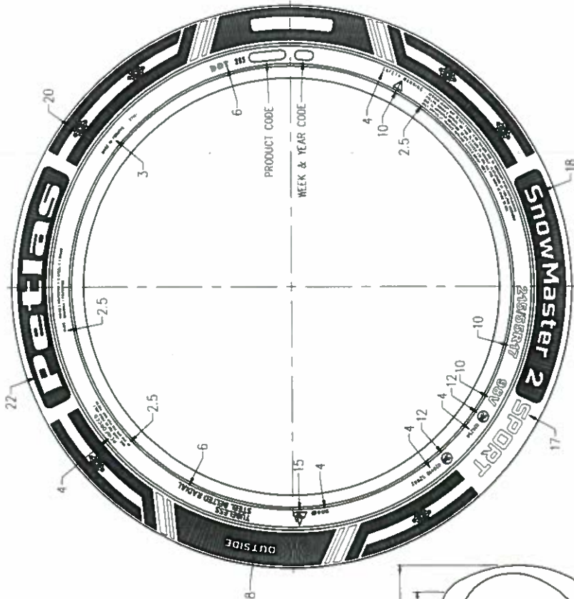
SERIAL SIDE
