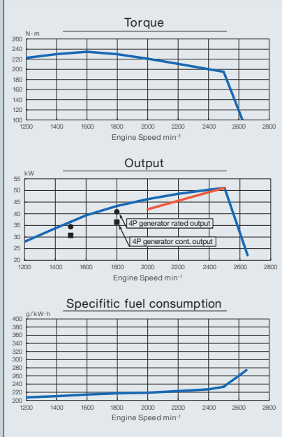
4TNV98-Z
