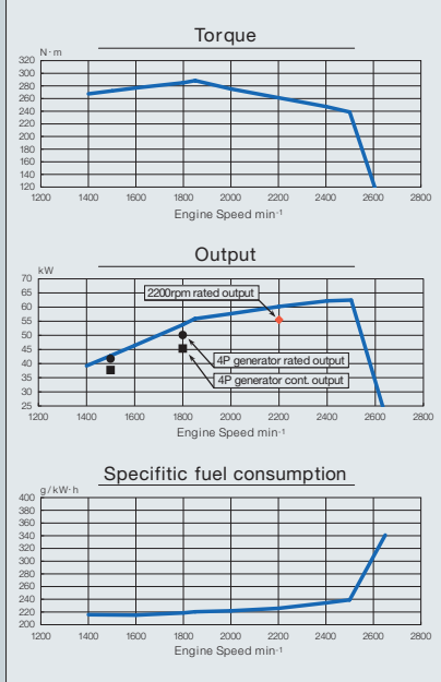
4TNV98T-Z
