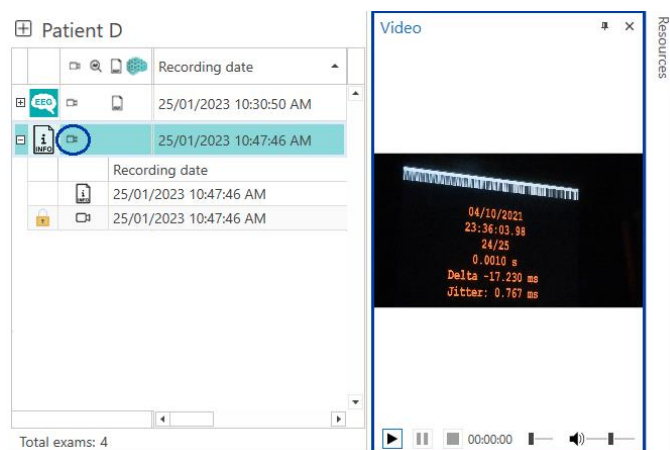
Video Panel
