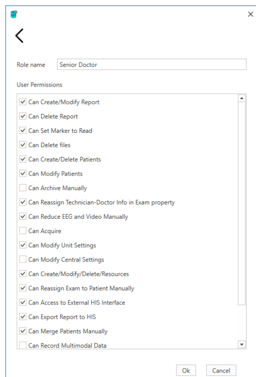
Role Permissions
