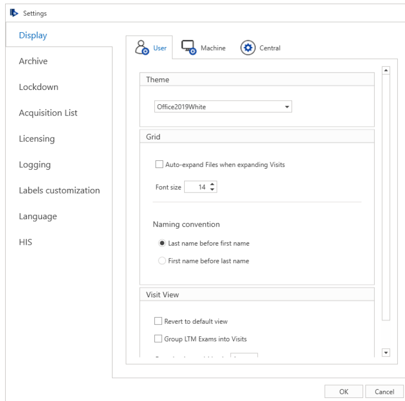
Settings window
