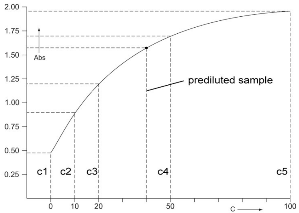
Fig.A-4 Interpolation on a calibration curve
