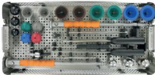
EcoFit® cup EPORE Container 02200036
