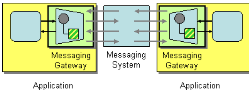
Figure 1: Messaging Gateway EIP
