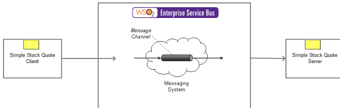
Figure 2: Example Scenario of the Message Channel EIP
