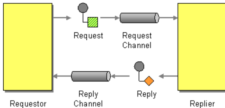
Figure 1: Request-Reply EIP
