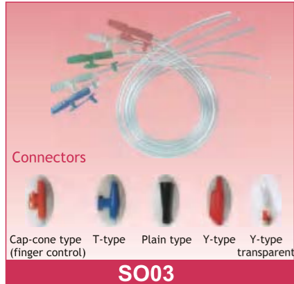
SO03 Suction Catheter Size: 5Fr-24Fr With or without detectable X-ray Polybag or blister packing
