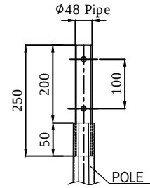
SPIGOT DETAIL
