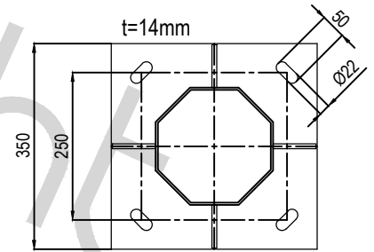
BASE PLATE
