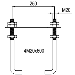
ANCHOR BOLT
