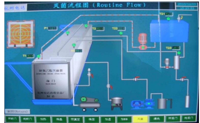
Sterilization Flow
