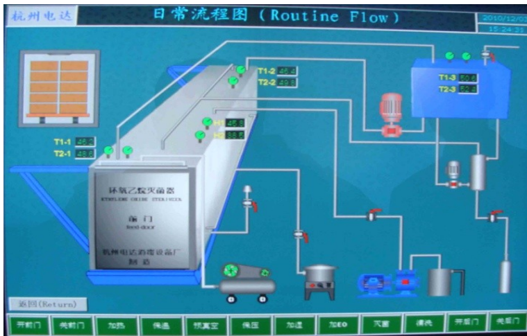
Pre-conditioning Flow
