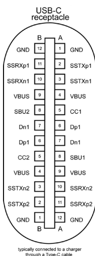
Figure 8. USB-C port
