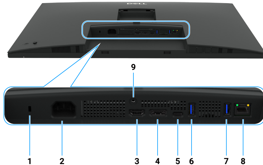
Figure 4. Bottom view of the monitor
