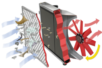
Normal operation.
