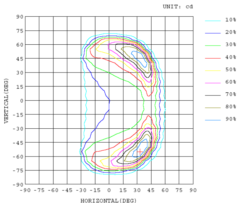
Diagrama Isocandela
