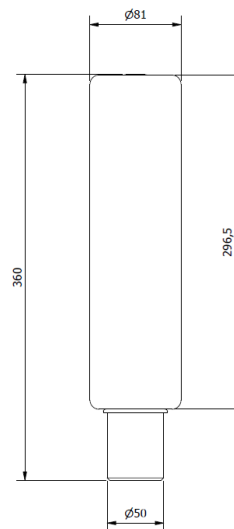
Resistance roll (4-09-100-09)
