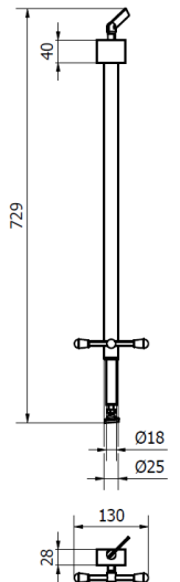
Support for arms of orthopaedic attachment (4-09-122)
