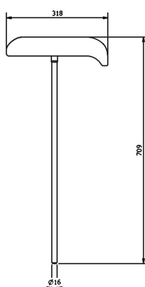
Foot support (4-09-102)
