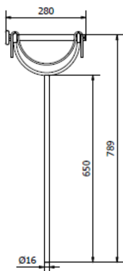
Bar support (4-09-101)
