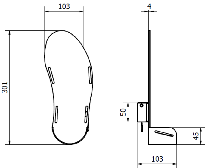
Foot support (4-09-108)
