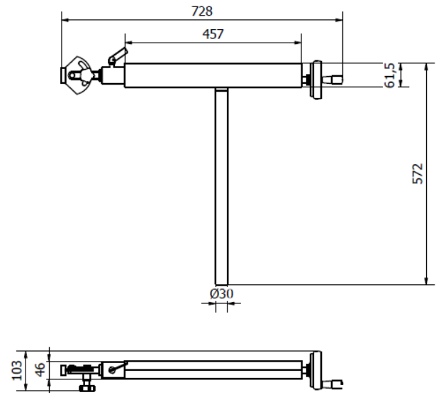
Traction mechanism (4-09-107)
