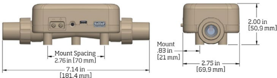
5300 Series Dimensions
