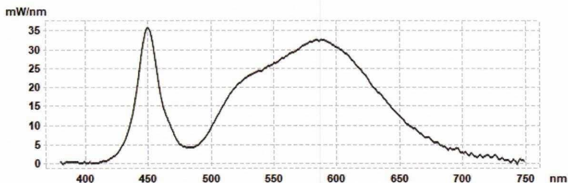
Spectral distribution
