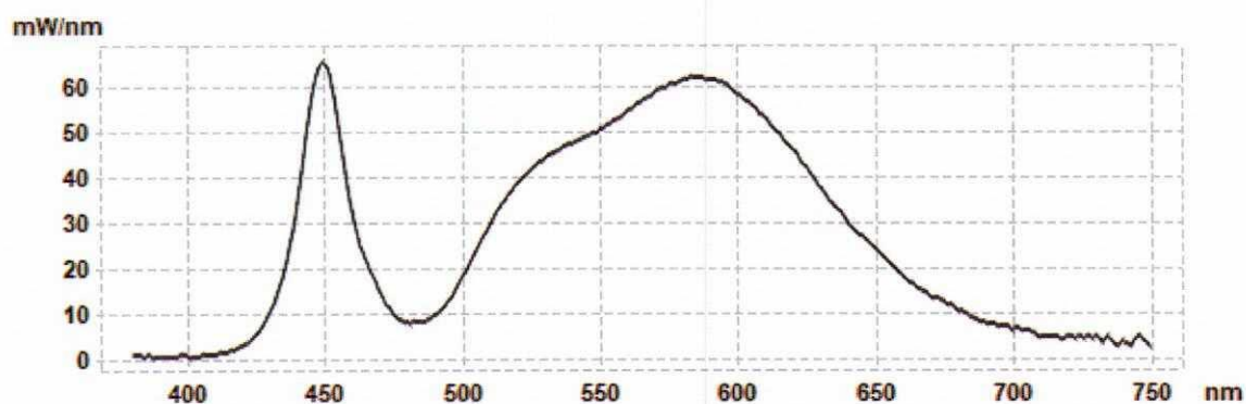
Spectral distribution
