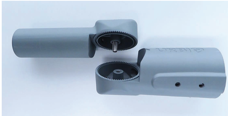
Console mechanism
