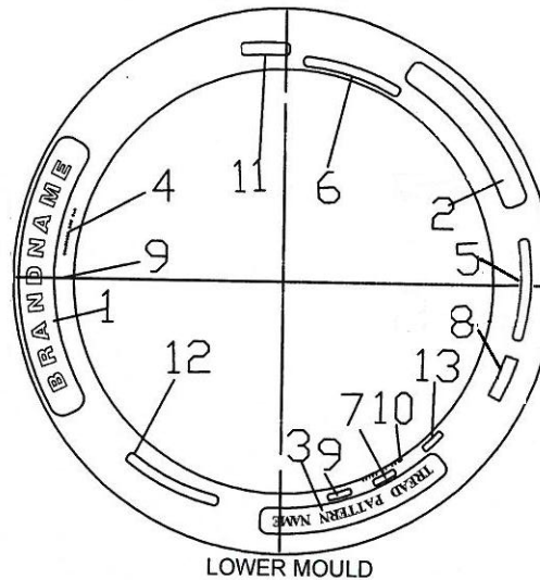
LOWER MOULD
