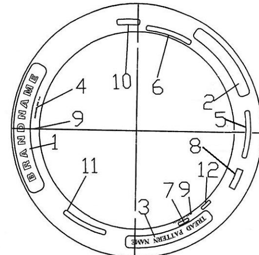
UPPER MOULD
