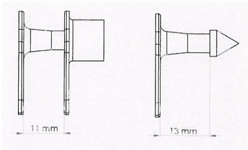
Multiflex L/L, distance and pin length
