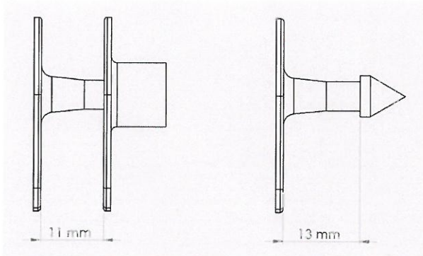
Multiflex P/P, distance and pin length
