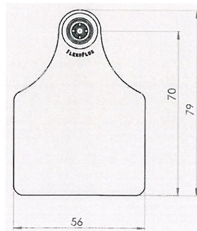
FlexoPlus D, mother part, dimensions
