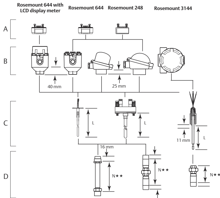
Figure 7: Sensor Assembly Without Thermowell
