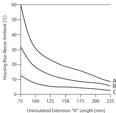
Figure 3: Transmitter Housing Temperature Rise vs. Uninsulated Extension Length
