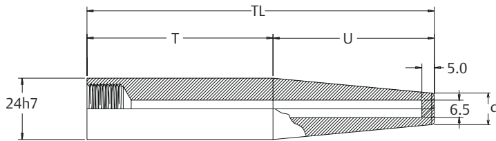
Figure 16: Weld-in Barstock Thermowell (Codes E01, E02, E04, E05)
