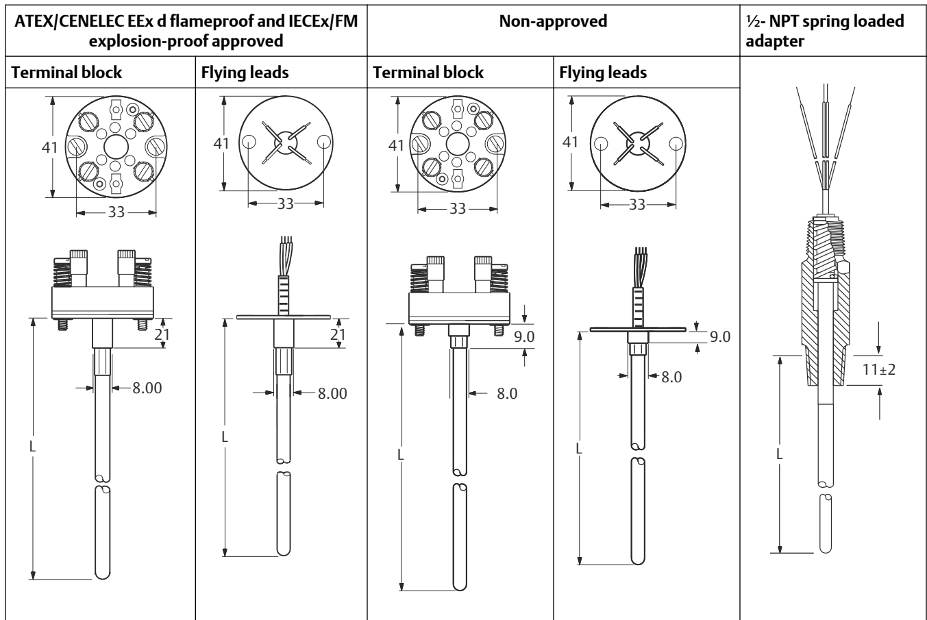
Figure 8: Series 65 RTD and Series 185 Thermocouple Dimensional Drawings
