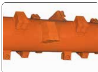
Rotore a denti fissi con riporti al tungsteno. Rotor, fixed teeth with tungsten coating and rotor with steel profiles.
