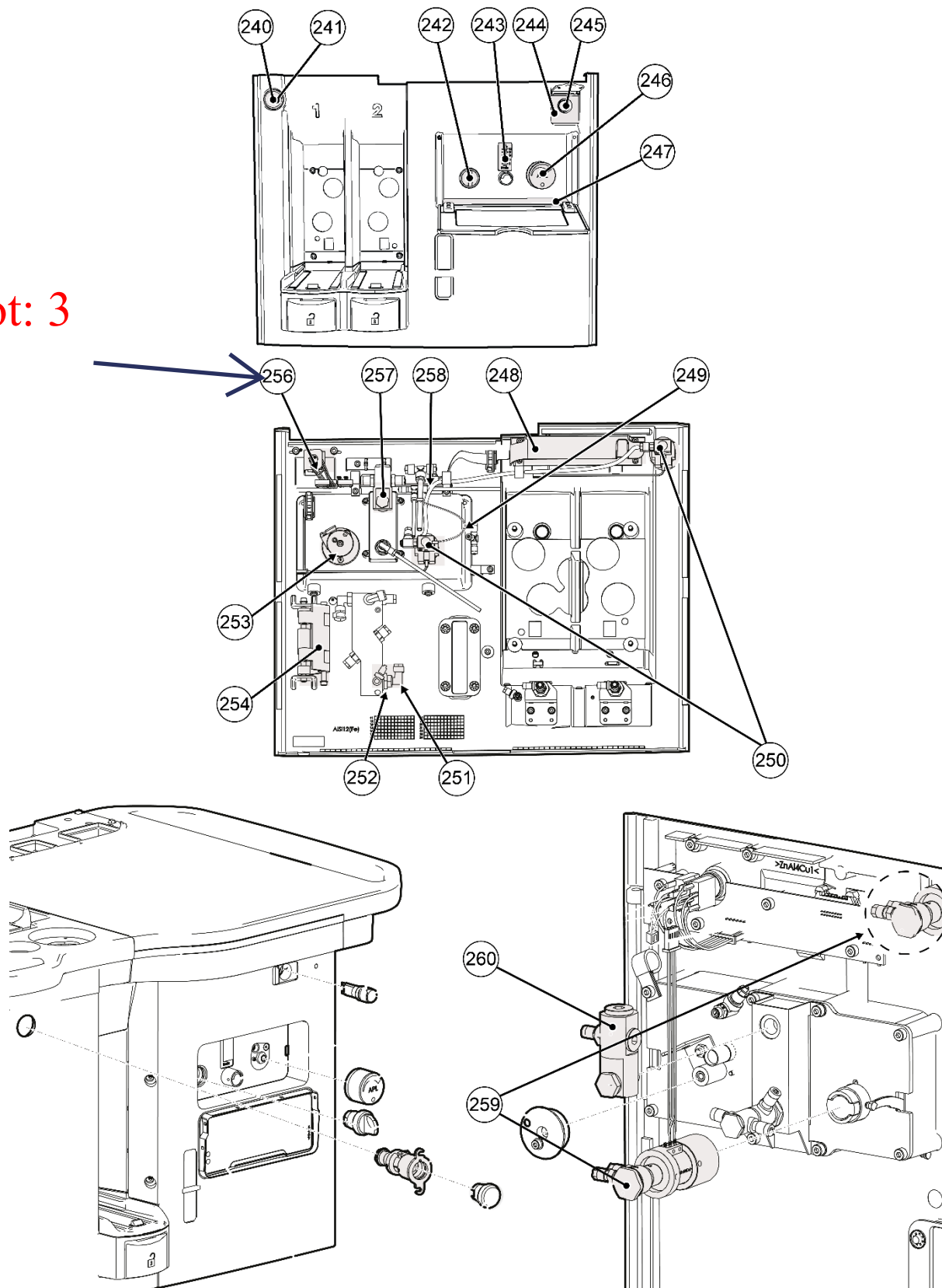
Figure 9: O 2 Flush/Emergency ventilation
