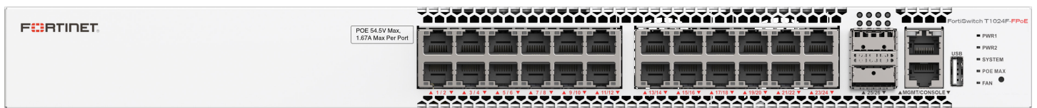
FortiSwitch-T1024F-FPOE — Front
