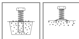
A concrete anchor B flat anchor
