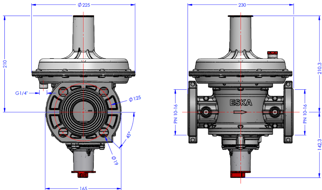
Figure 7: ERG-EH DN50 Flanged Technical Dimensions
