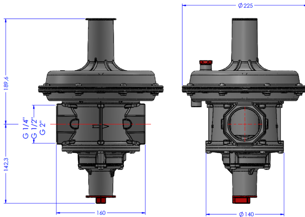
Figure 6: ERG-EH Technical Dimensions
