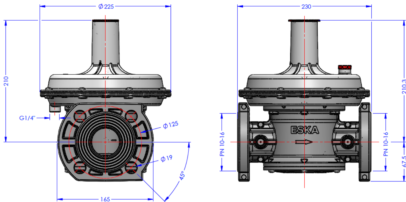
Figure 8: ERG-H DN50 Flanged Technical Dimensions
