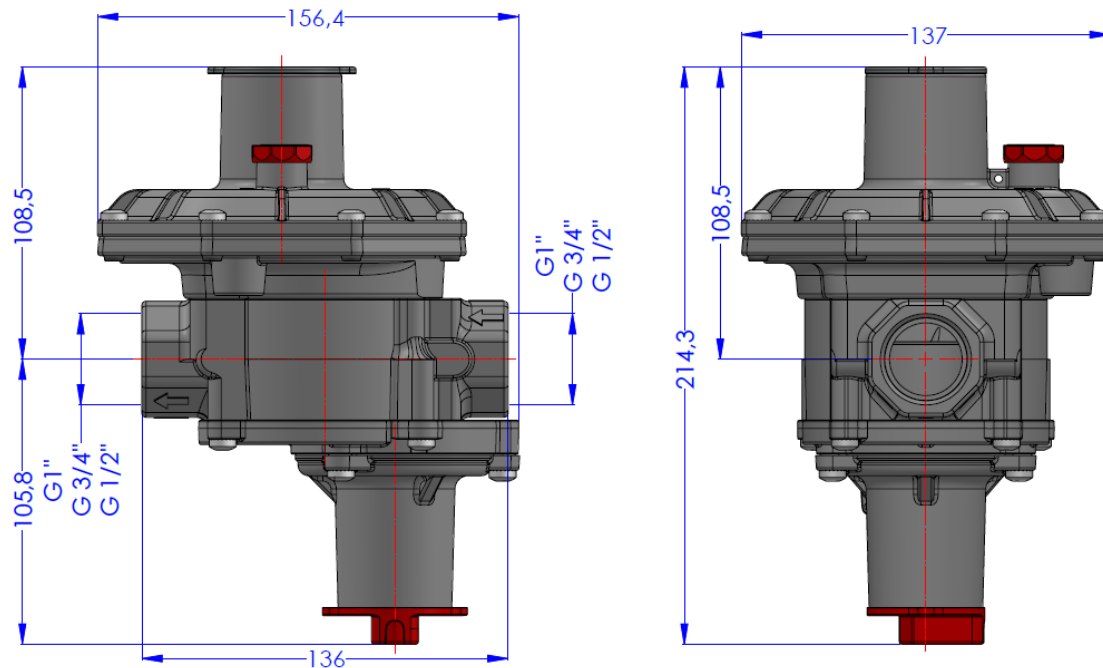
Figure 5: ERG-EH Technical Dimensions
