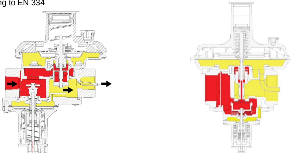
Figure 2: ERG-EH Pressure Display
