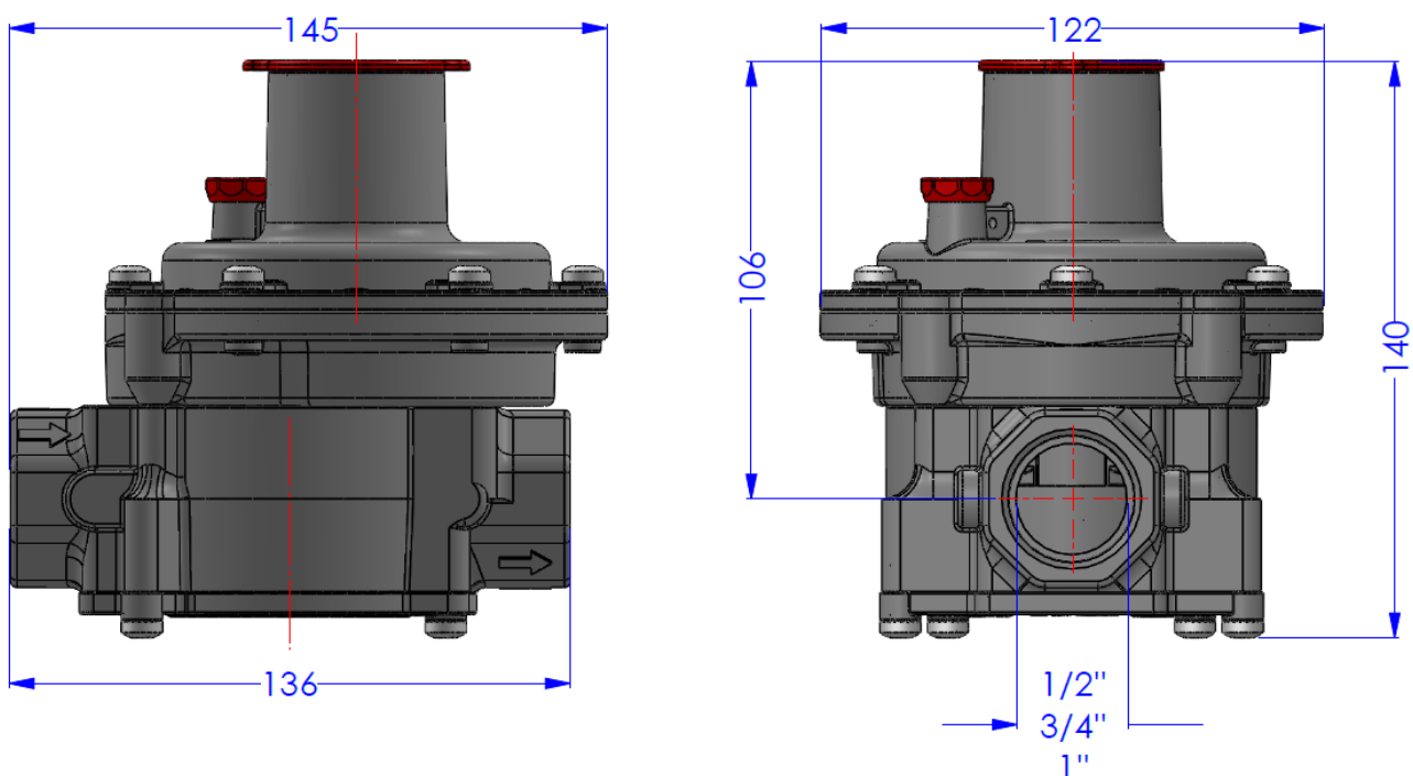
Figure 9: ERG-H Technical Dimensions
