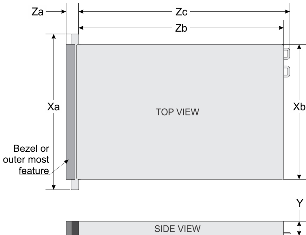
Figure 41. Chassis dimensions
