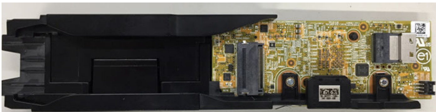
Figure 20. BOSS-N1 Controller
