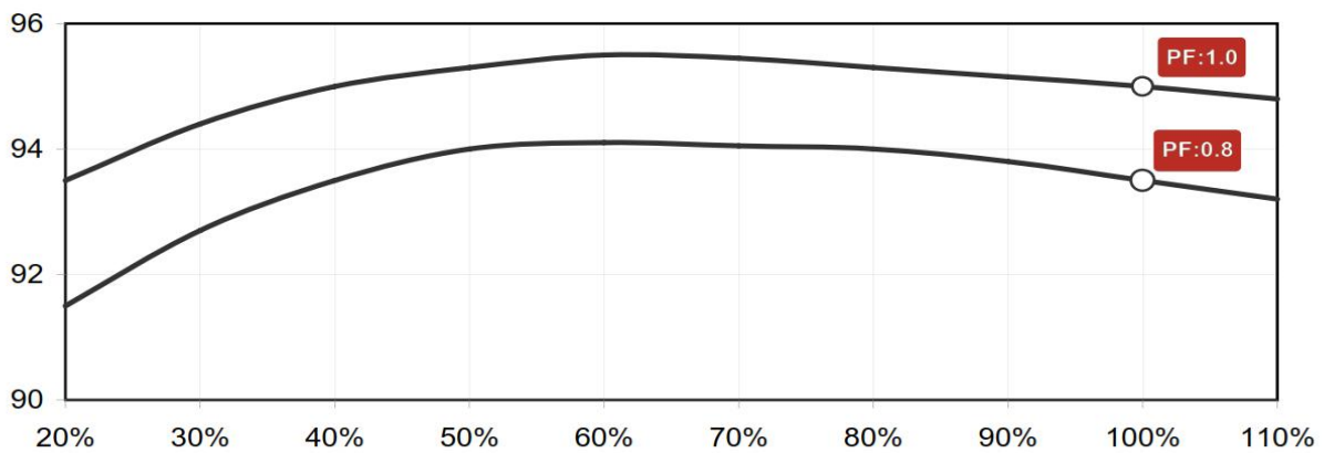
Efficiency Curves @ 60 Hz, 480V
