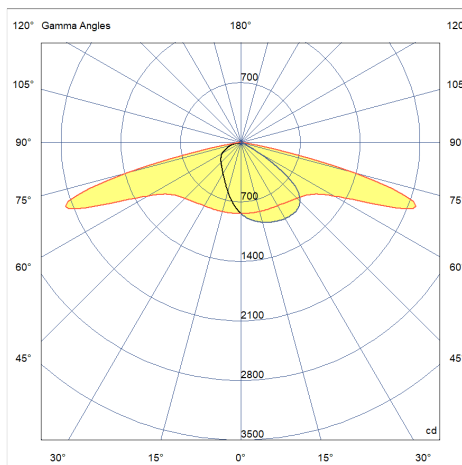
CRIOTEK 01 LED 19.8W ASTRO
