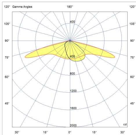
CRIOTEK 01 LED 10.4W ASTRO
