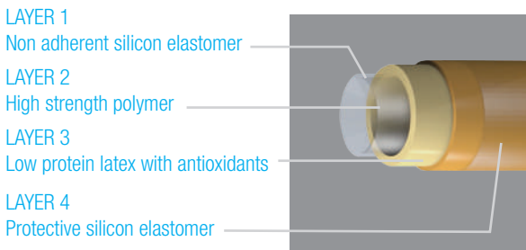
Unique Four Layer System
