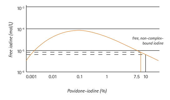
Fig 1. Equilibrium concentrations of povidone-iodine
