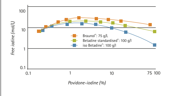
Fig 2. Free iodine concentration in aqueous povidone-iodine-solutions
