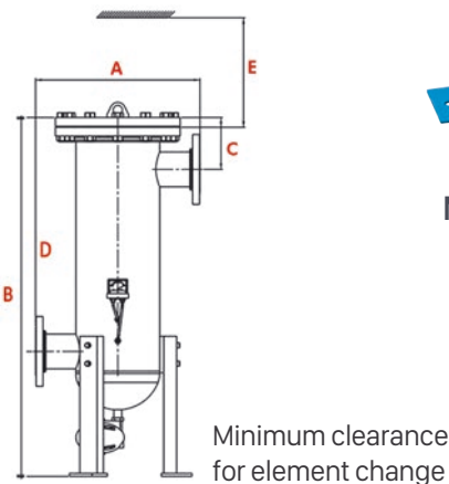
Minimum clearance for element change
