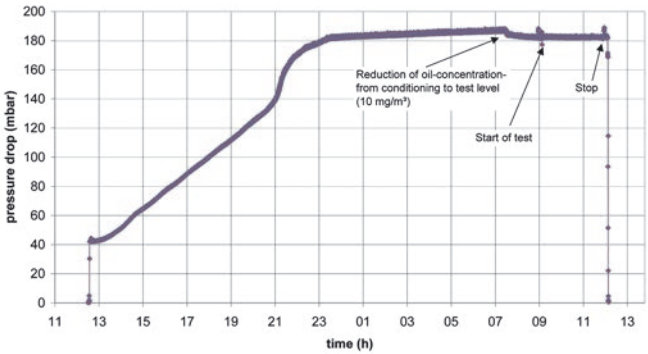
Drytec M50Y-2 at 50 m³/h ANR - 7 bar(e) 28.-29.09.10
