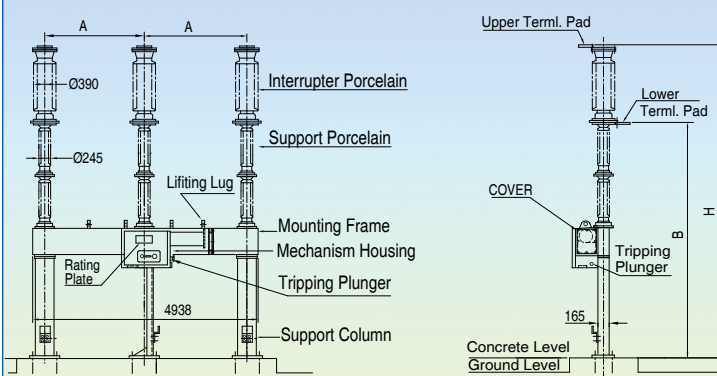
170kV Single Phase Auto Reclosing Breaker
