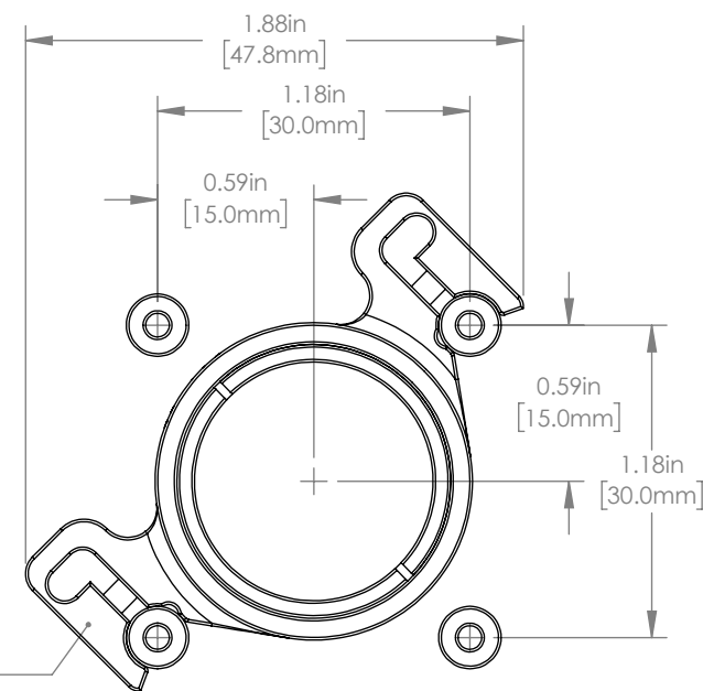
MOUNTED VIEW 30mm CAGE SYSTEM (ER RODS NOT INCLUDED)
