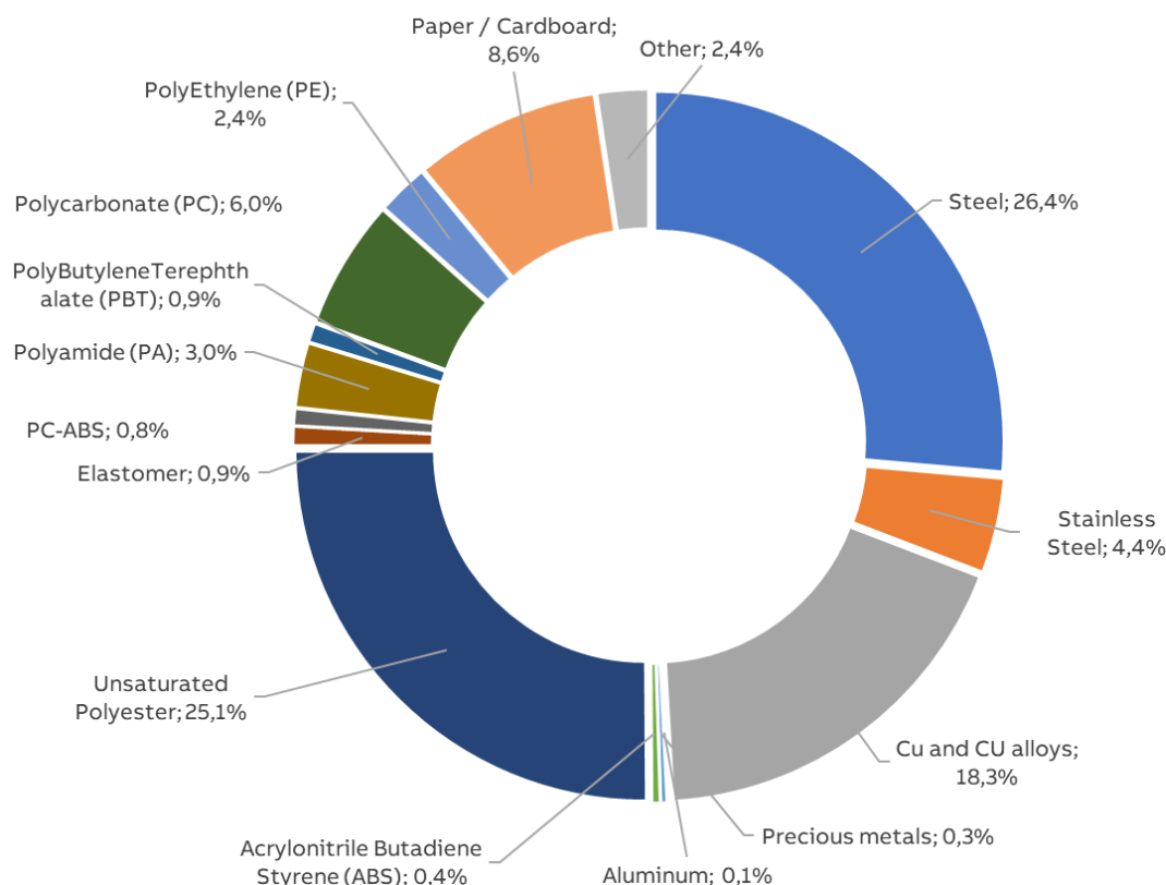
Figure 1: Composition of XT5 3p IEC N/S/H/L Ekip DIP 400A
