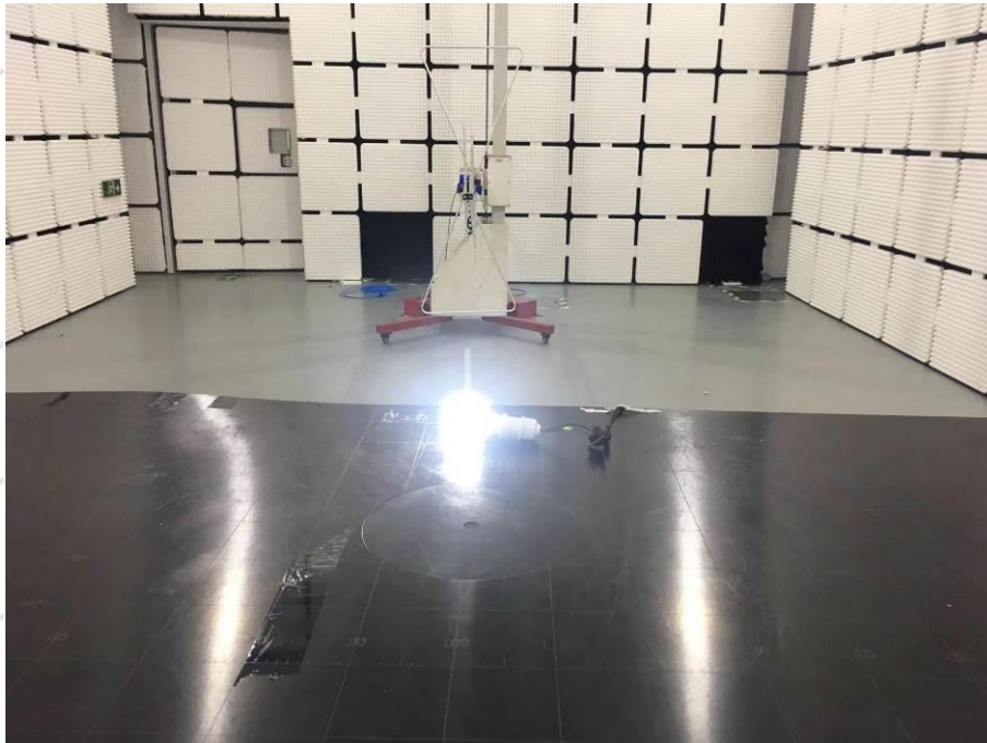
Photo 6 Radiated Emission Test
