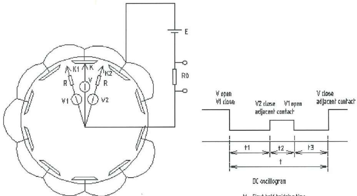
DC oscillographic measurement circuit
