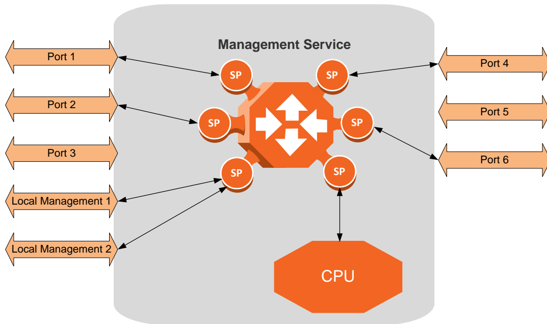
Figure 84: Management Service
