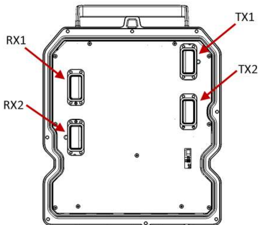
Figure 21: RFU-D-HP Radio Interfaces
