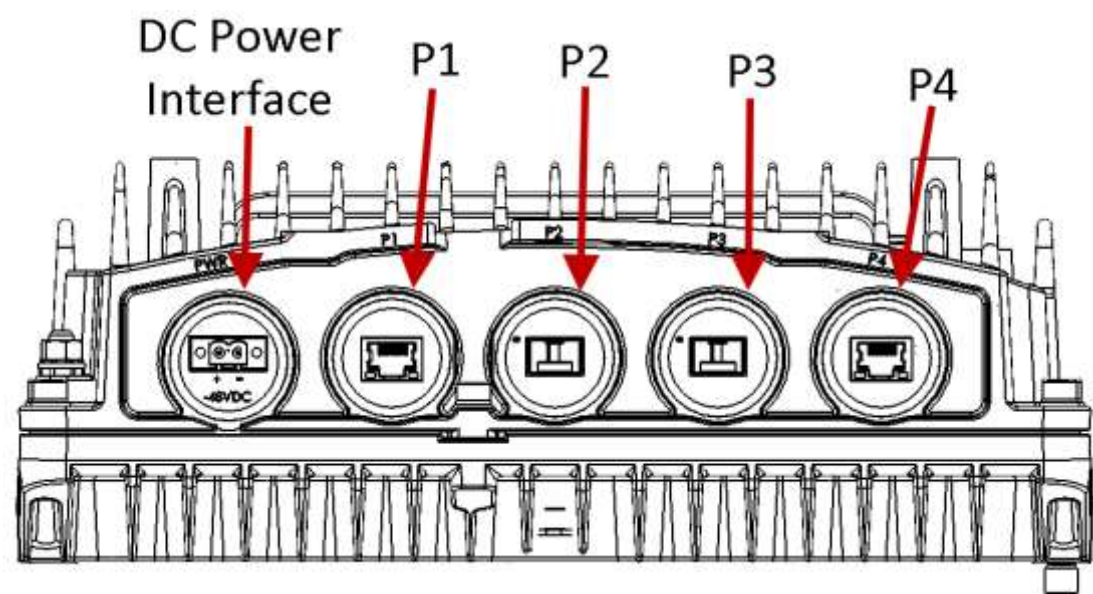
Figure 23: RFU-D-HP Interfaces
