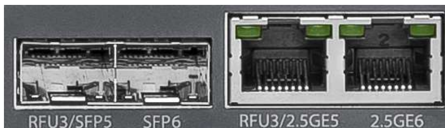
Figure 3: RFU3/SFP5-6 Interfaces
