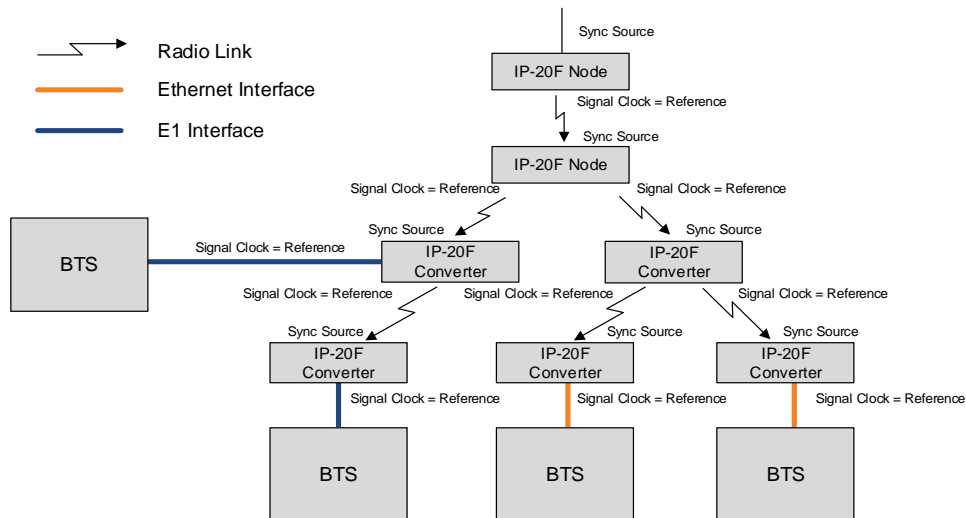
Figure 112: Synchronization Configuration
