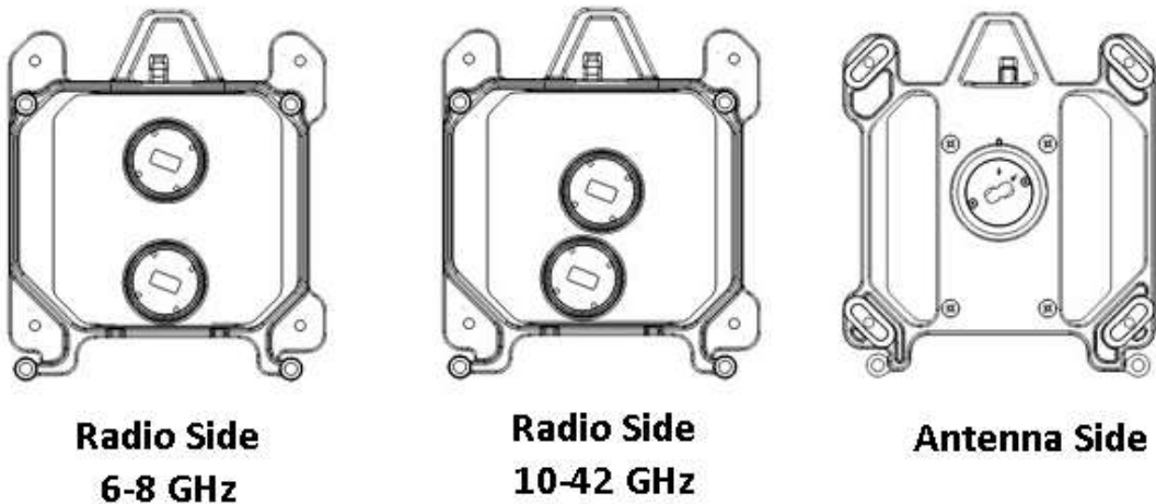
Figure 18: Splitter
