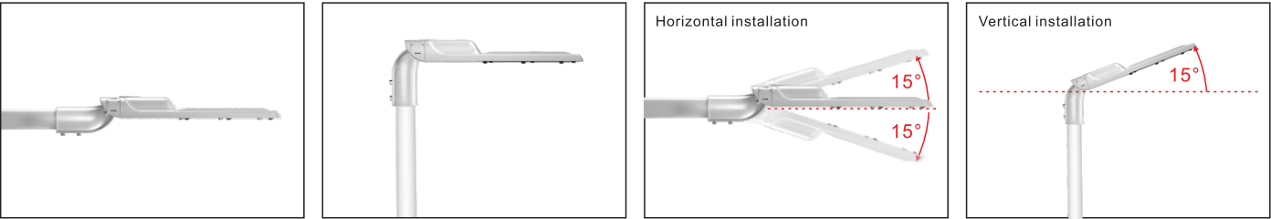
Horizontal installation
