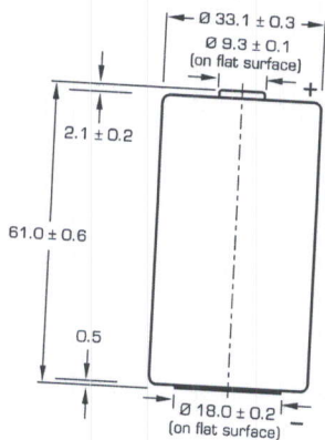
Finished version with protruding positive end cap
