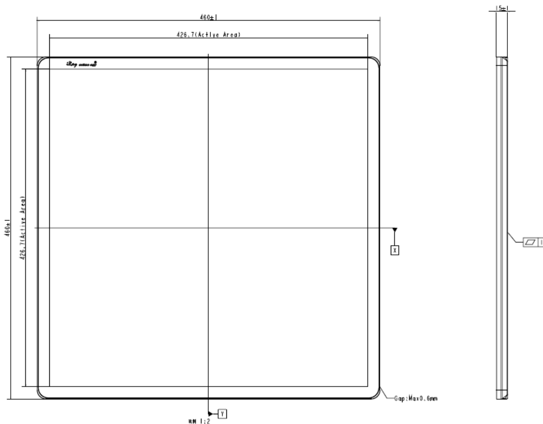
Fig1. Detector Mechanical Outline (unit:mm)
