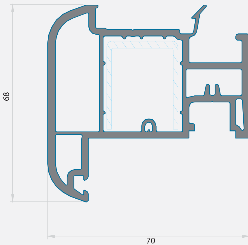
■ F60000 - MULLION PROFILE
