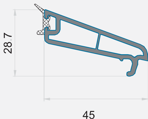
■ F42000 - GLAZING BEAD PROFILE, 5 mm
