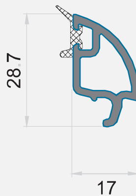
■ F40000 - GLAZING BEAD PROFILE, 32 mm
