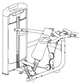
CONVERGING SHOULDER PRESS
