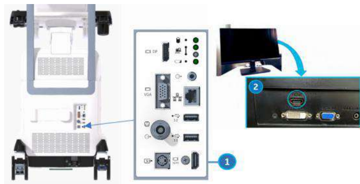
Figure 3-7. Connect HDMI Cable to back of LOGIQ Totus and External Monitor
