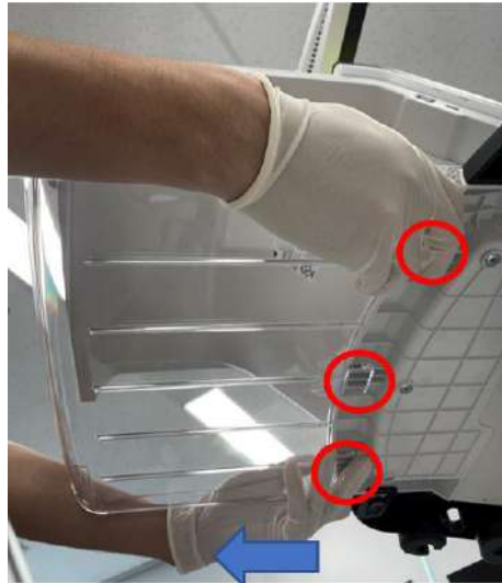
Figure 12-14. Disassemble the Control panel rear tray
