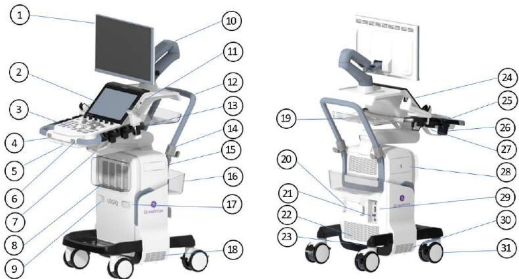
Figure 3-1. LOGIQ Totus System
