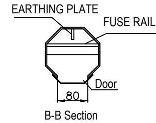
B-B Section
