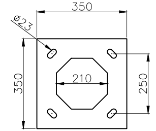
BASE PLATE # 14 mm x 350x 350
