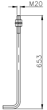
4 x M20 x 720 Anchor Bolts
